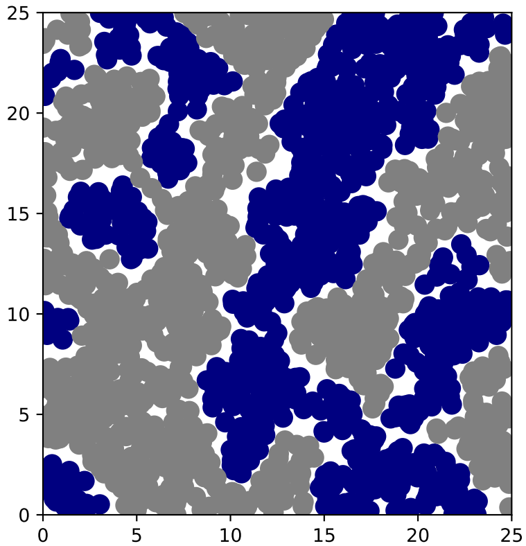
Widom-Rowlinson model with two-color intensity 0.04
